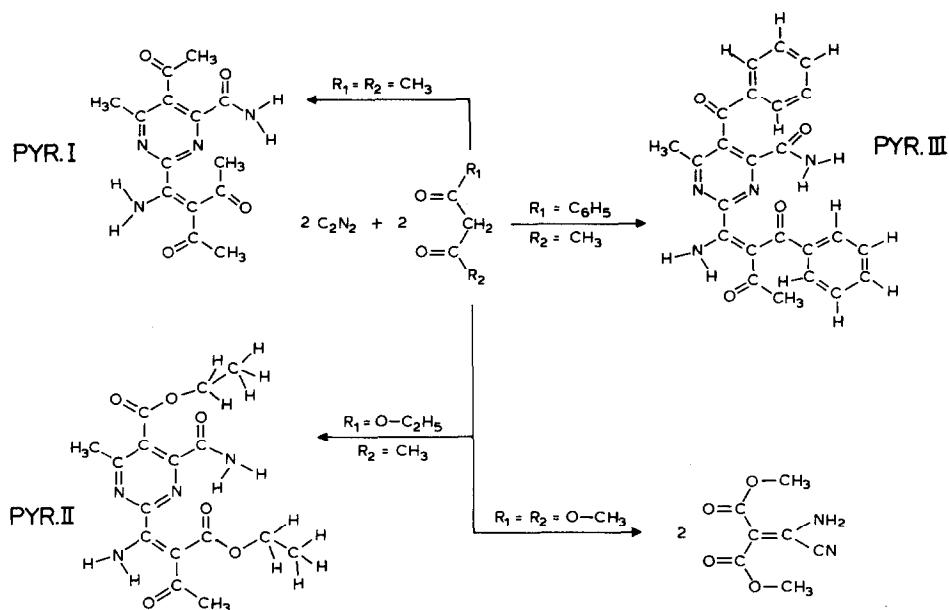
Scheme 10. The cyanation of \beta -dicarbonylic compounds catalyzed by [\text{Ni}(\text{acac})_2]
