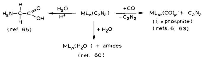
Scheme 2. Reactions of coordinated \text{C}_2\text{N}_2
